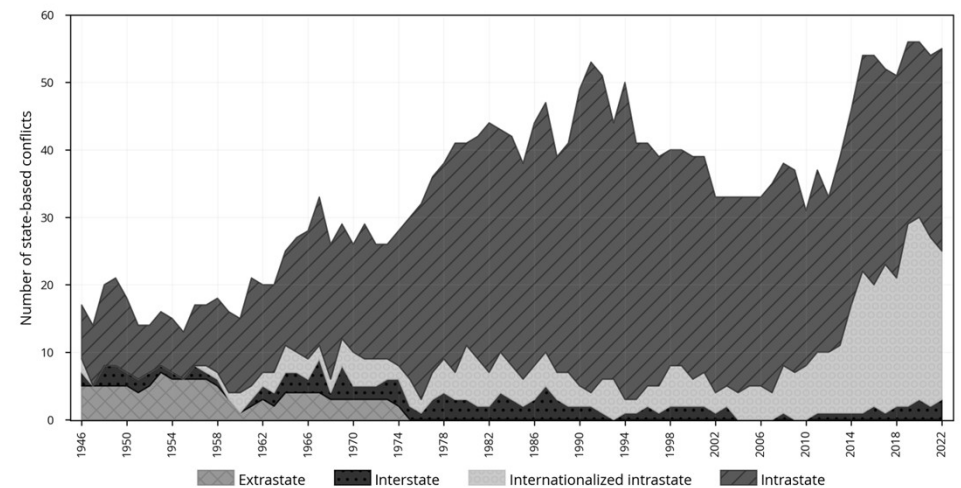
State-based conflicts by type of conflict (1946-2022)
